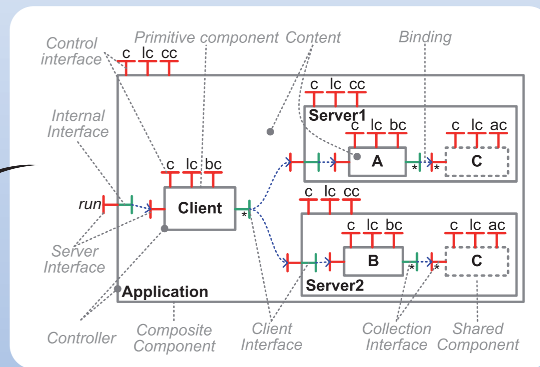
Fractal - A modular and reflective component model
