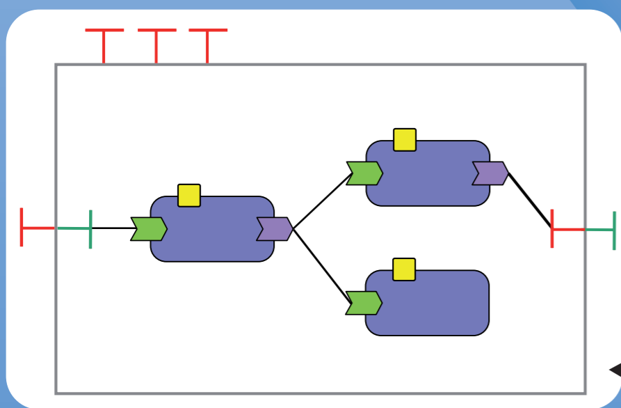
Reconfigurable SCA Applications
