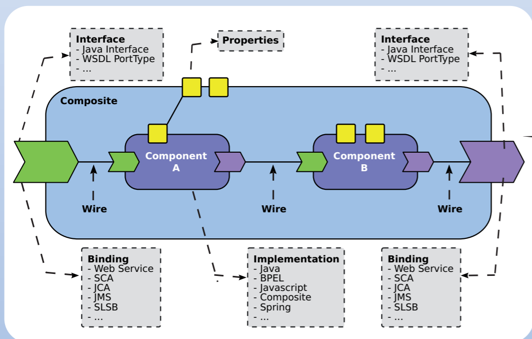
SCA - The standard component model for SOA
